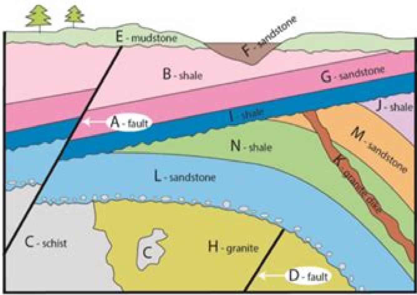
Figure 1. Geological cross-section. Illustration by K. Wiese
