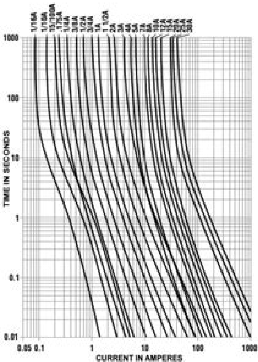
Slow Blow Fuses
