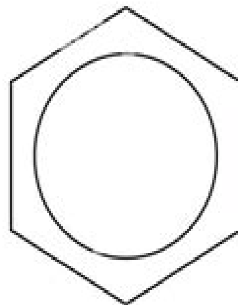
Hexagon with pi electron delocalization
