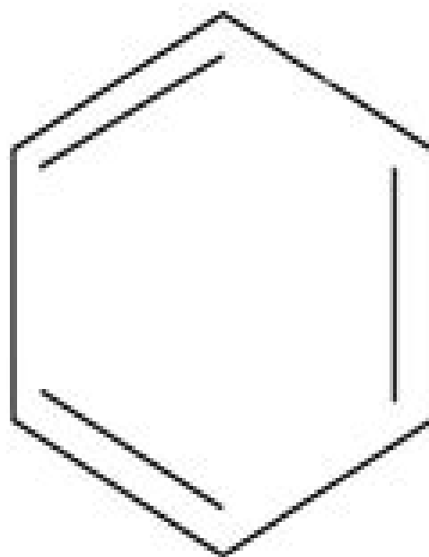
Hexagon with 3 pi bonds
