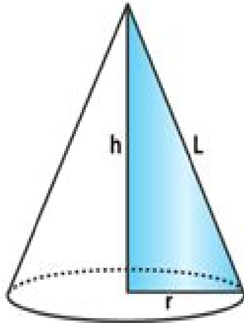
Right circular cone
