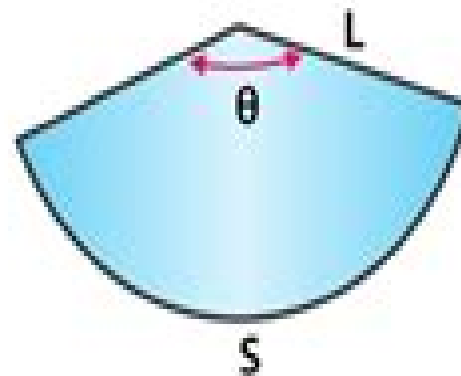
Unrolled lateral area
