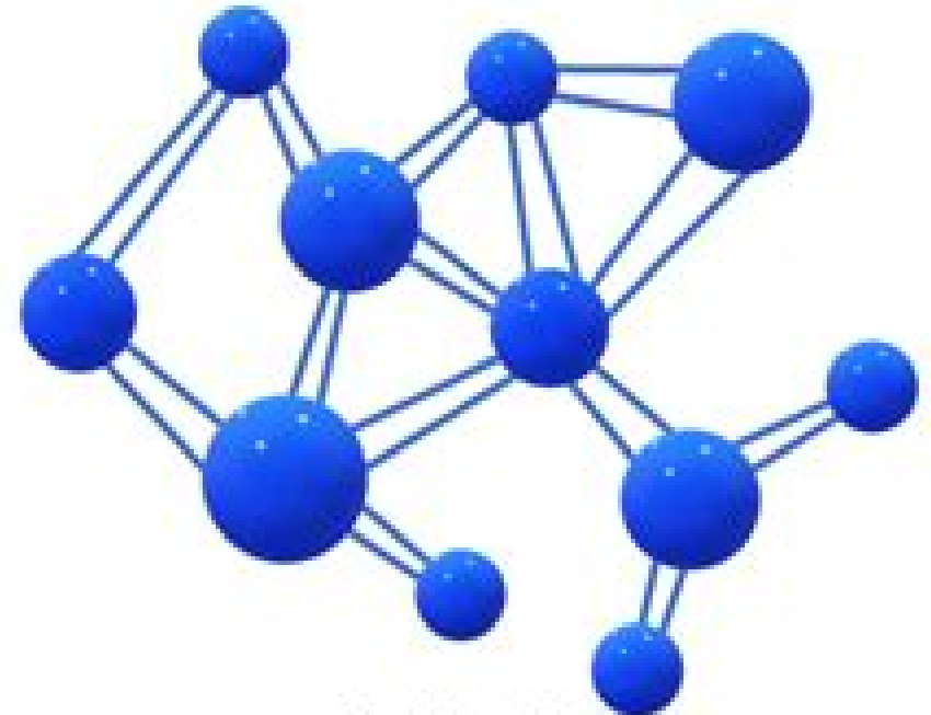
Networked Polymers
