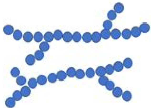
Branched Polymers
