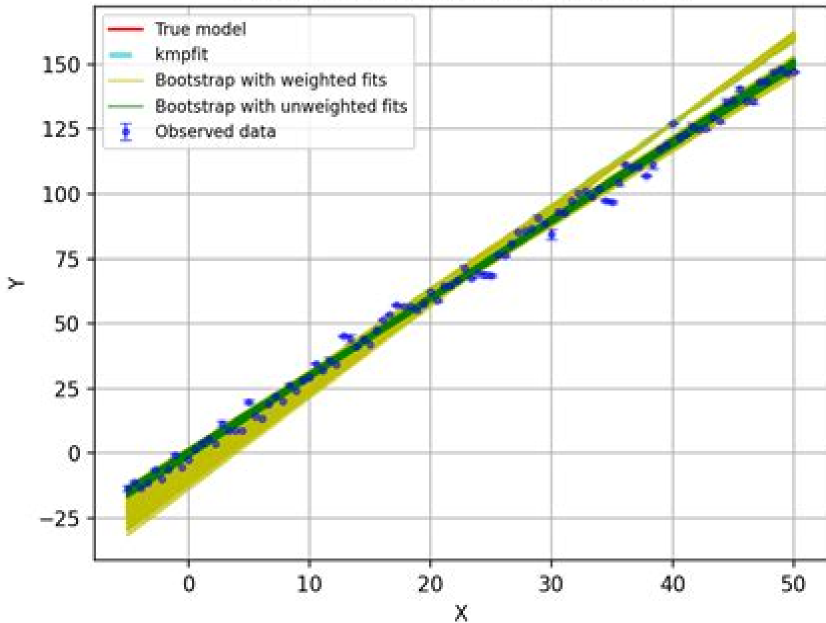
Bootstrap with weighted and unweighted fits
